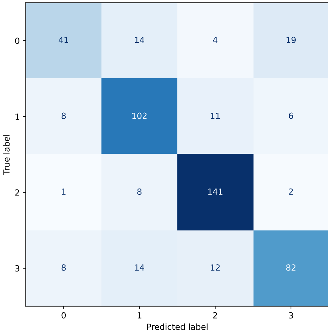
STFT Confusion Matrix
