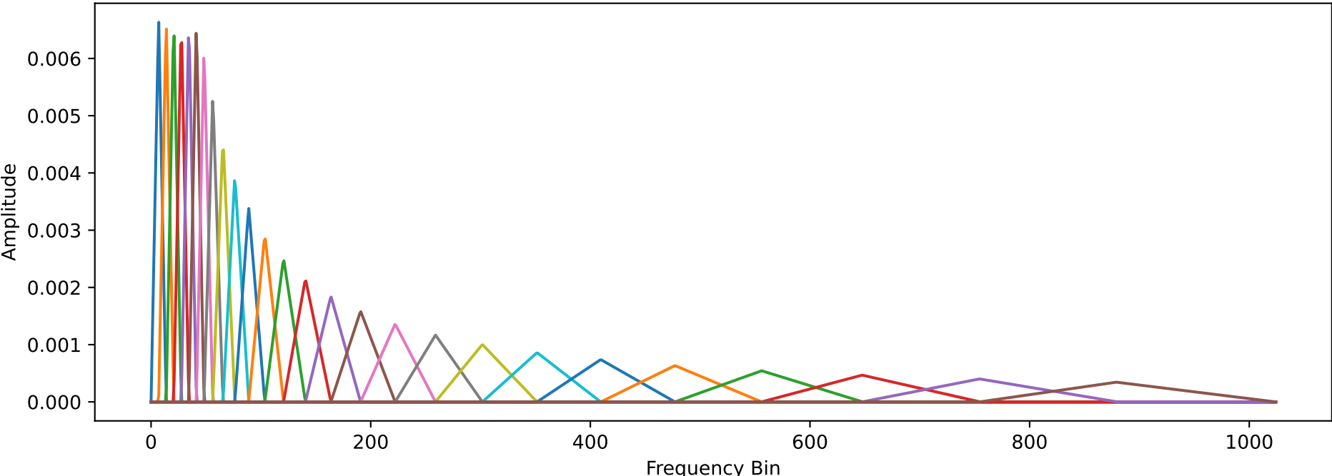
Mel Filter Bank
