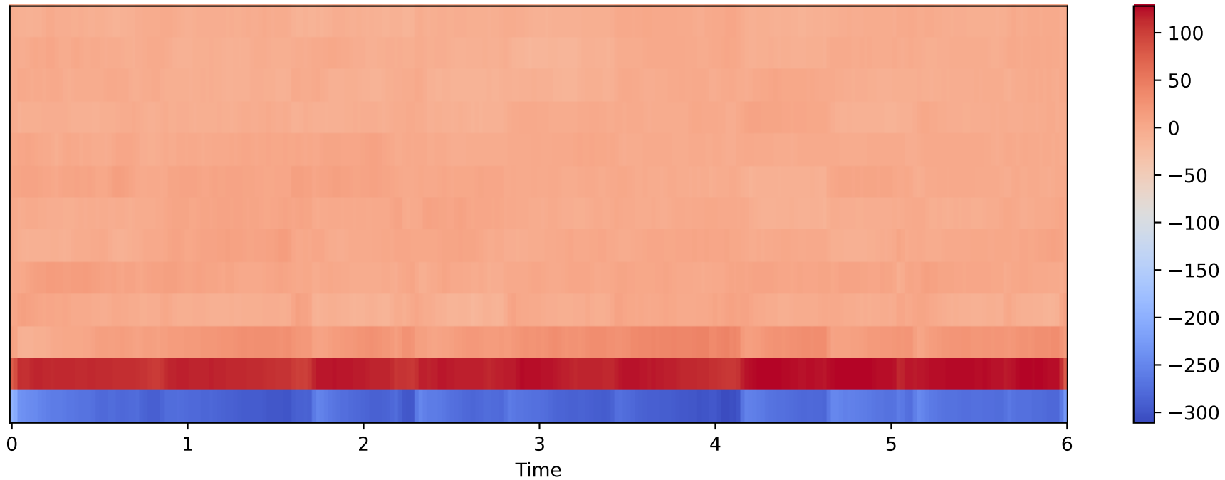
MFCC
