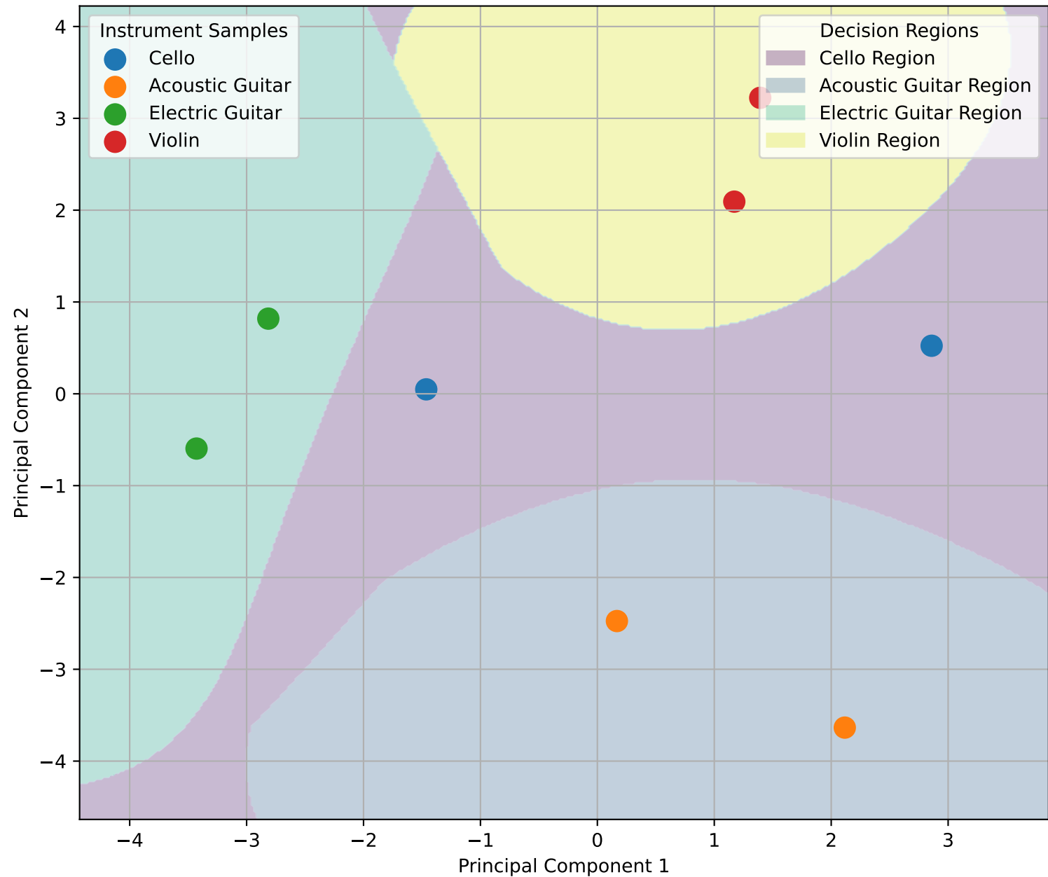
SVM Decision Regions
