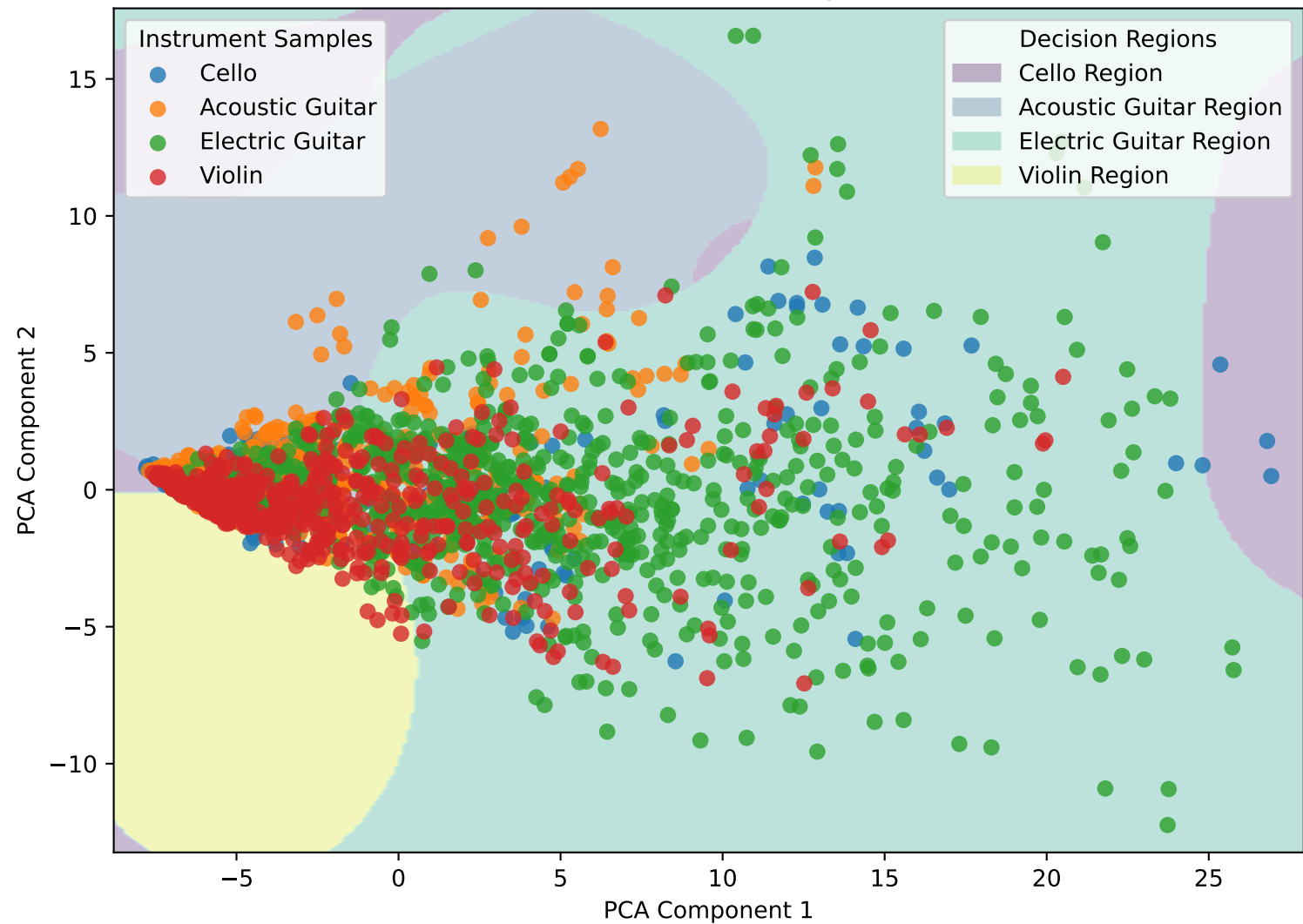
CQT SVM Decision Regions
