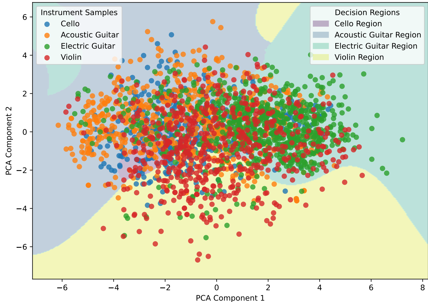
MFCC SVM Decision Regions
