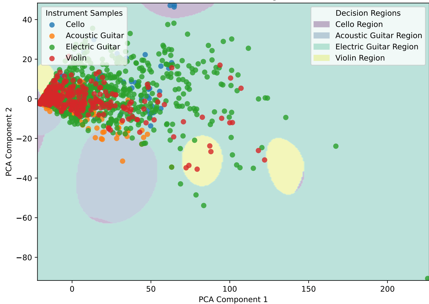
STFT SVM Decision Regions
