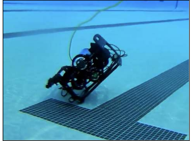
Fig. 7. Picture of Sea++'s during an underwater trial
