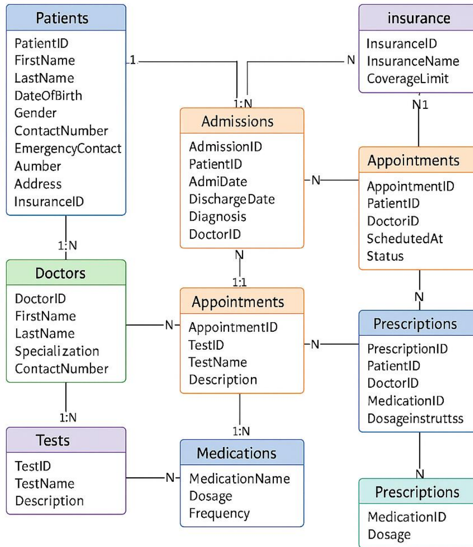
Figure 1: Entity-Relationship diagram depicting the alternate schema with colored entities and cardinalities.
