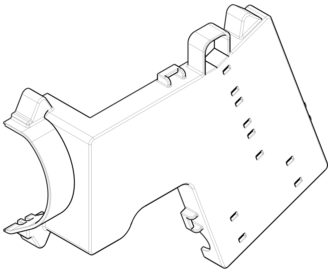
ISO VIEW SCALE 1:1
