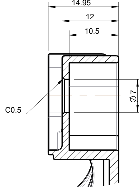
SECTION E-E
