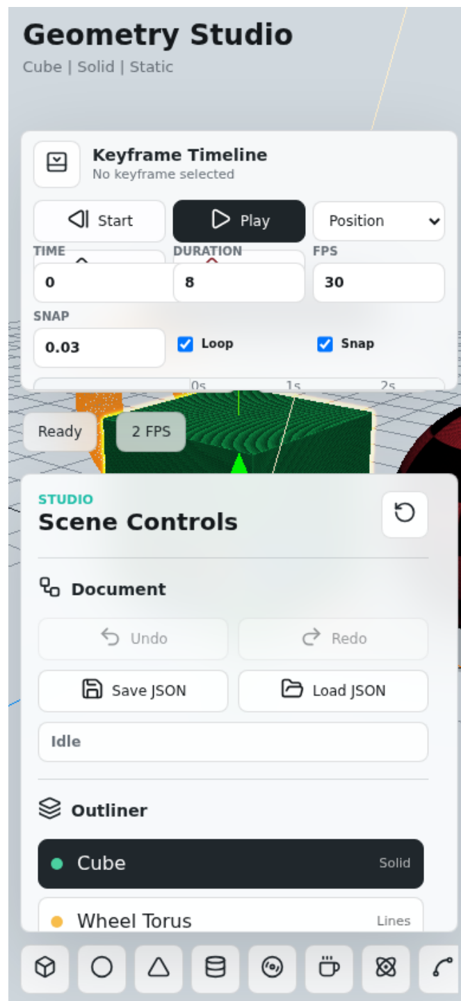
Figure 9: Responsive mobile layout with timeline, inspector, viewport, and horizontal tool rail.
