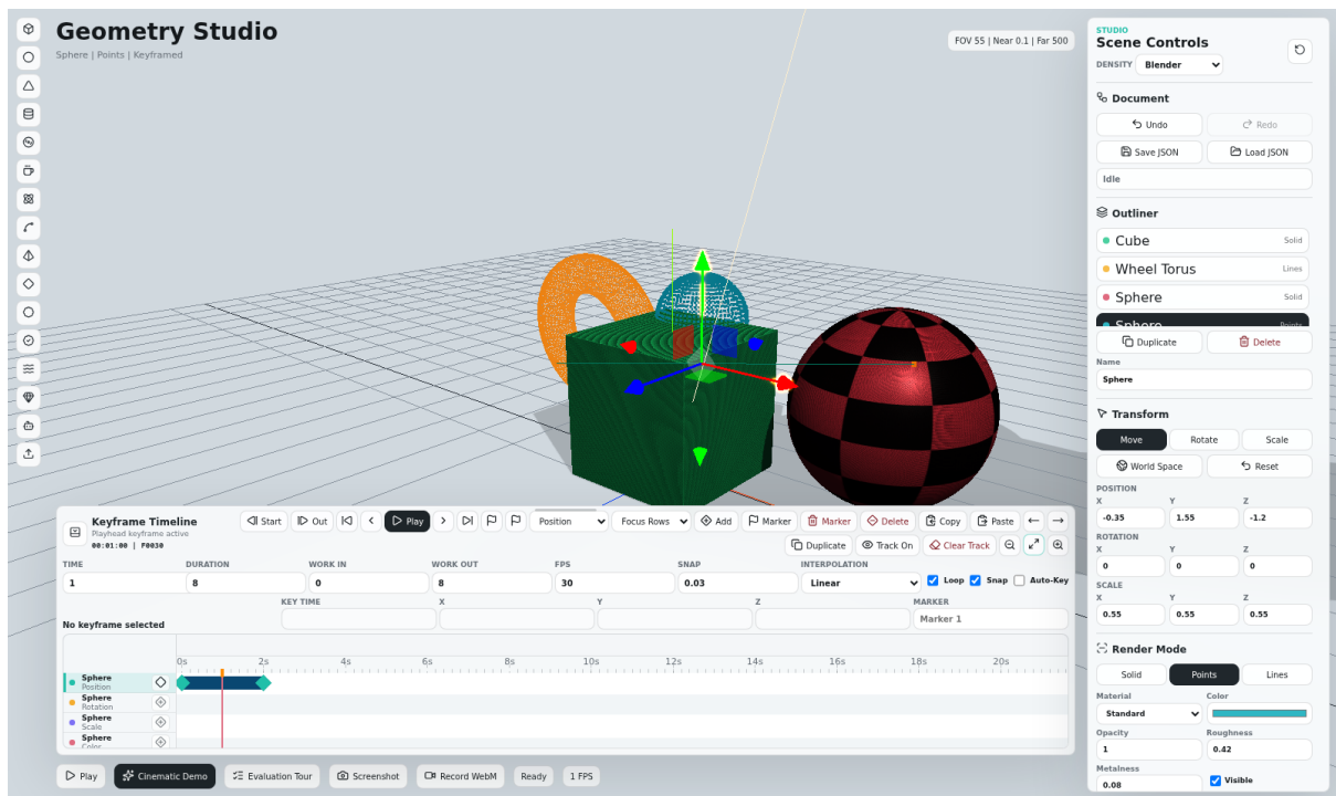
Figure 10: Position keyframes with the selected object's viewport motion path, showing the spatial interpolation from one keyed position to the next.
