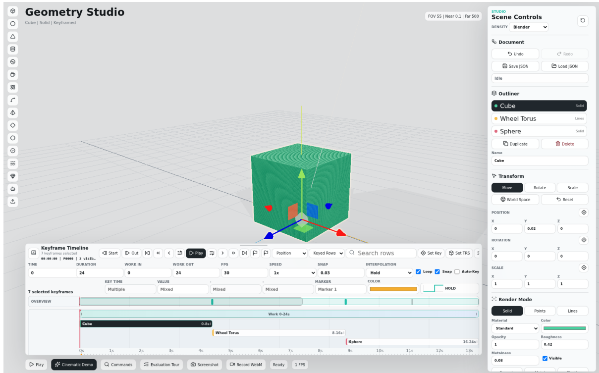
Figure 7: Sequenced object layer ranges showing staged object visibility, expanded duration, selected Visibility keys, and shifted object animation keys.
