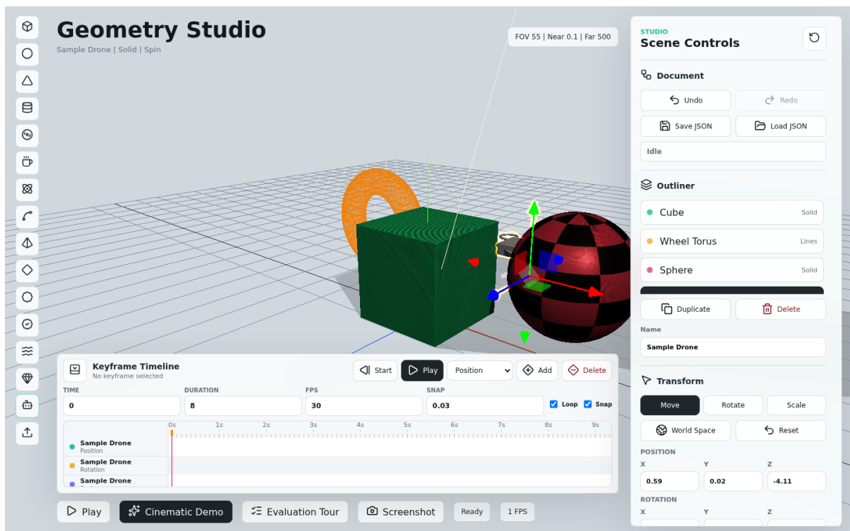
Figure 8: Built-in sample model workflow demonstrating model-style objects in the same outliner, transform, render, and animation system.
