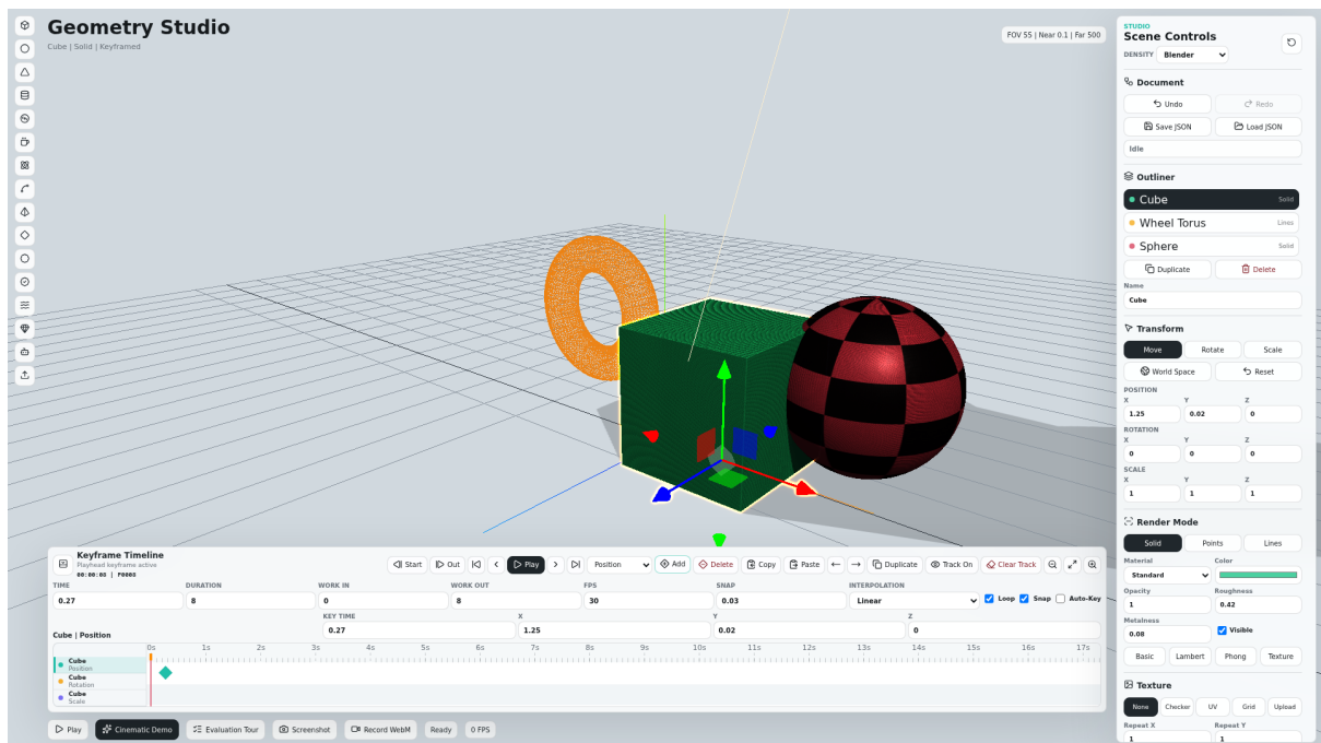
Figure 4: Transform keyframe timeline showing two Position keyframes and a selected object whose X position was keyed through the timeline workflow.
