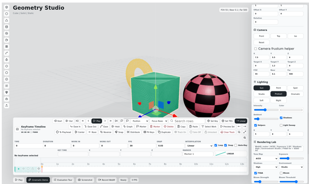
Figure 9: Rendering Lab with Product lighting, FXAA, SSAO, tone mapping, environment lighting, and the direct-light preset controls visible in the inspector.
