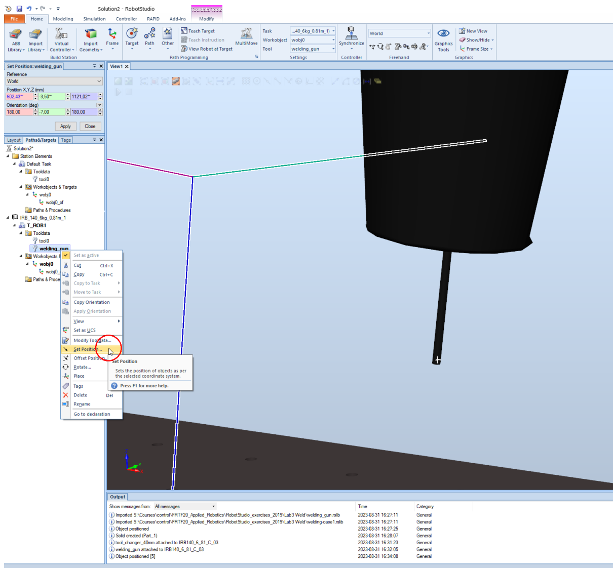
Figure 4: Setting the position of the welding gun tip reference frame
