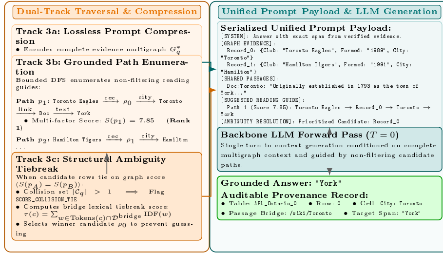
Fig. 3. Detailed illustration of OUEG dual-track reasoning, structural ambiguity resolution, and unified prompt payload. (Left) Rather than destructive top- N path filtering, Track 3a compresses the complete evidence subgraph with a shared passage dictionary \mathcal{S}_p , while Track 3b enumerates multi-factor scored candidate paths ( S(p) ) as non-filtering reading guides. Track 3c detects structural candidate score collisions, applying a bridge lexical tiebreak \tau(c) to resolve ties deterministically. (Right) The synthesized compact prompt payload provides the backbone LLM with complete evidence and directed reading focus, producing the grounded answer alongside a full provenance trace.
