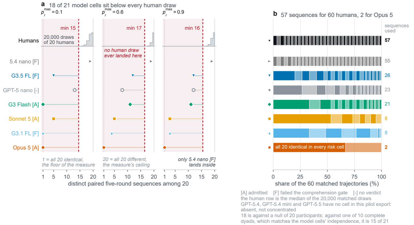
Figure 4: Human participants use far more of the policy space than any checkpoint here. Panel a places each checkpoint’s count of distinct paired five-round action sequences against 20,000 draws of twenty human participants, matched on sample size and risk condition; the shaded region is the range no human draw ever reached. Eighteen of the twenty-one checkpoint cells fall below every human draw, so they have no percentile rather than a low one; against a stricter null built from ten complete human dyads, which matches the checkpoints’ unit of independence and not only their sample size, the count is fifteen. Panel b shows which sequences each population actually uses, with each checkpoint marked admitted, failed, or without a verdict by the endpoint-admission gate of Table 2. The one checkpoint that reaches the human range is the one that failed the gate. Three routes the nine-route baseline reports have no cell in this pilot export and are absent rather than concentrated.
