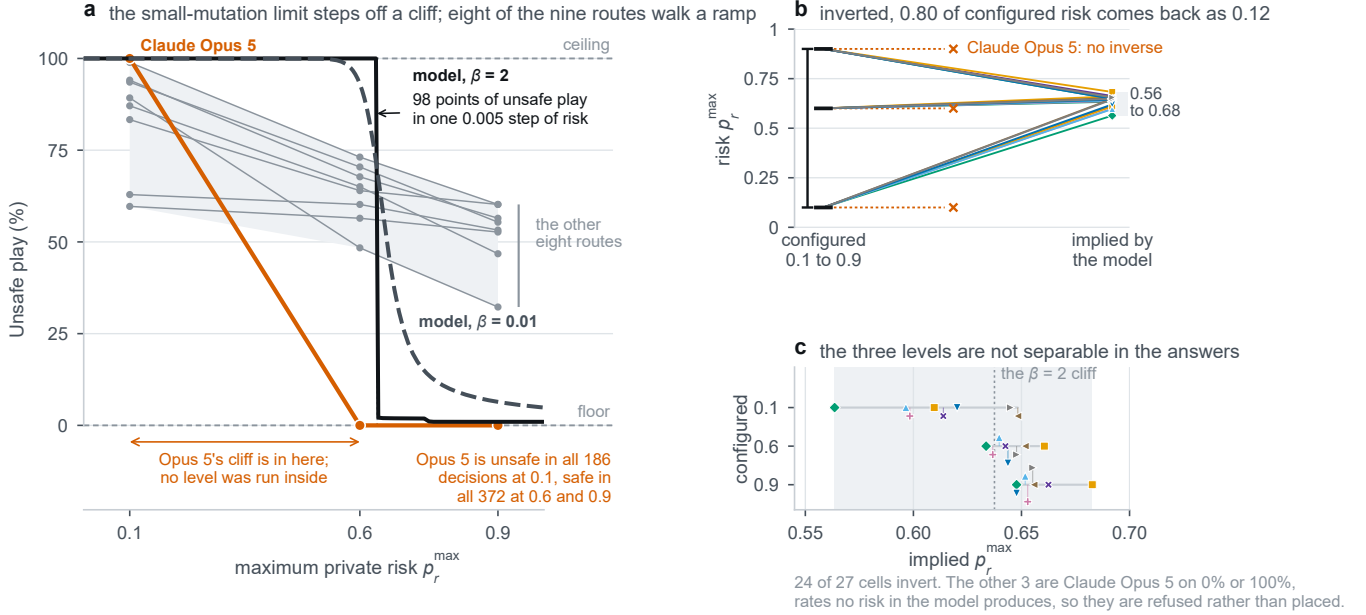
Figure 3: The reconstructed evolutionary benchmark and the audited routes have different shapes, not different levels. Panel a rebuilds the reduced game’s payoff matrix across a fine grid of risk values and solves the small-mutation limit at each, at both declared selection strengths; at \beta = 2 the predicted UNSAFE rate falls by 98 points inside a single 0.005 step of risk, while eight of the nine routes decline gradually across the whole range. Claude Opus 5 is the exception, drawn in its own colour: it does have a cliff, but no risk level was run inside the interval where it falls. Panel b inverts the model, asking which risk it would need to emit each observed rate; the configured range of 0.80 returns as a band of 0.12. Panel c shows the consequence: the three configured levels are not separable in the model’s answers. Every curve here is the small-mutation limit, which cannot represent the finite mutation rate of the parameter points it is drawn at, so this bounds the regime in which the benchmark is read and is not a test of the model.
