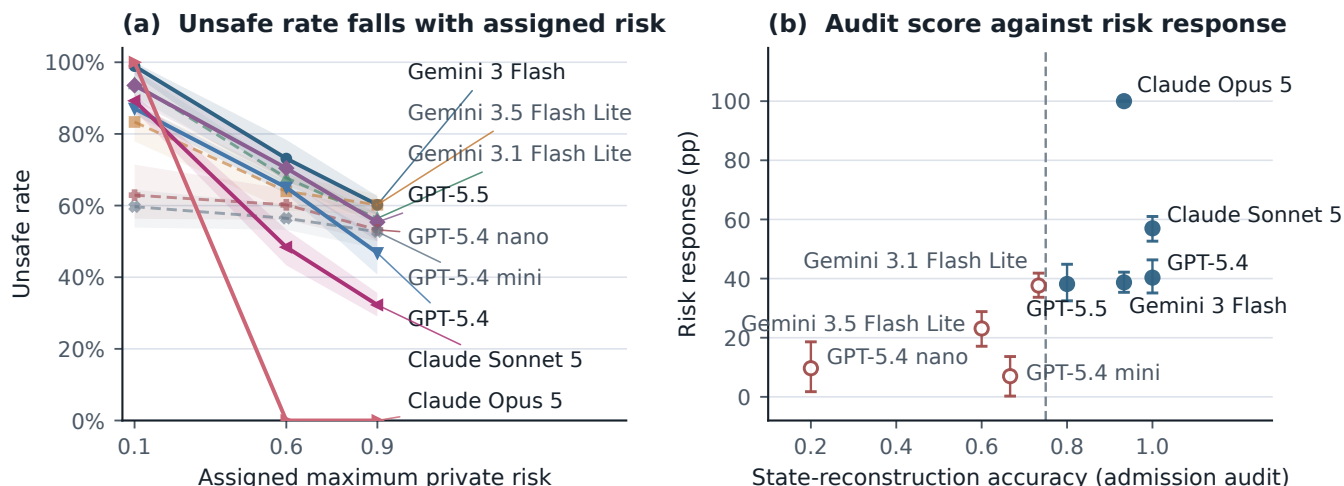
Figure 2: Measured comprehension against strategic sensitivity, over the nine audited routes, all of which completed the confirmatory baseline. (a) UNSAFE rate against assigned maximum private risk, with 95% race-clustered bootstrap bands; solid lines are admitted routes, dashed lines refused ones. (b) State-reconstruction accuracy against the risk response, the UNSAFE-rate difference between risk 0.1 and 0.9, with race-clustered intervals; filled points are admitted, hollow refused, and the dashed rule is the 75% admission threshold. Claude Opus 5 is a degenerate step policy with zero within-cell variance and is reported as a boundary case.
