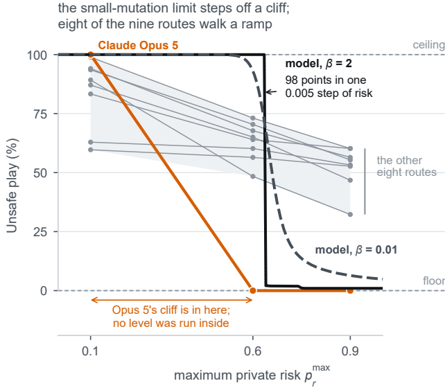
Figure 3: The evolutionary benchmark and the audited routes differ in shape, not level. The small-mutation limit is solved on a fine grid of risk values at both declared selection strengths: at \beta = 2 the predicted UNSAFE rate falls 98 points inside one 0.005 step, while eight routes decline gradually. Claude Opus 5, in its own colour, does have a cliff, but no risk level was run inside the interval where it falls, and its two saturated cells have no room beside them: it plays UNSAFE on all 186 decisions at risk 0.1 and SAFE on all 372 above it. Every curve is the small-mutation limit, which cannot represent the finite mutation rate of the points it is drawn at, so this bounds the regime in which the benchmark is read and is not a test of the model. The supplementary material inverts that model through these rates, which is a question about the model rather than about the routes.
