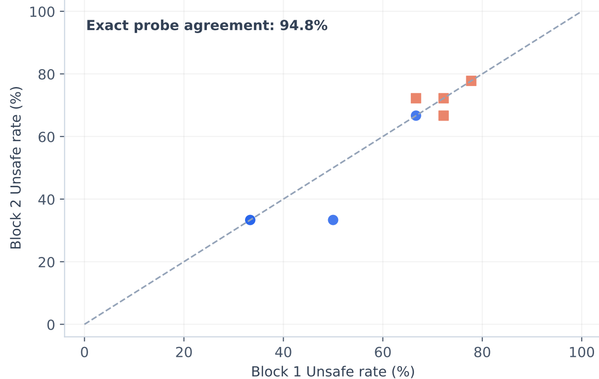
Qwen2.5-7B
