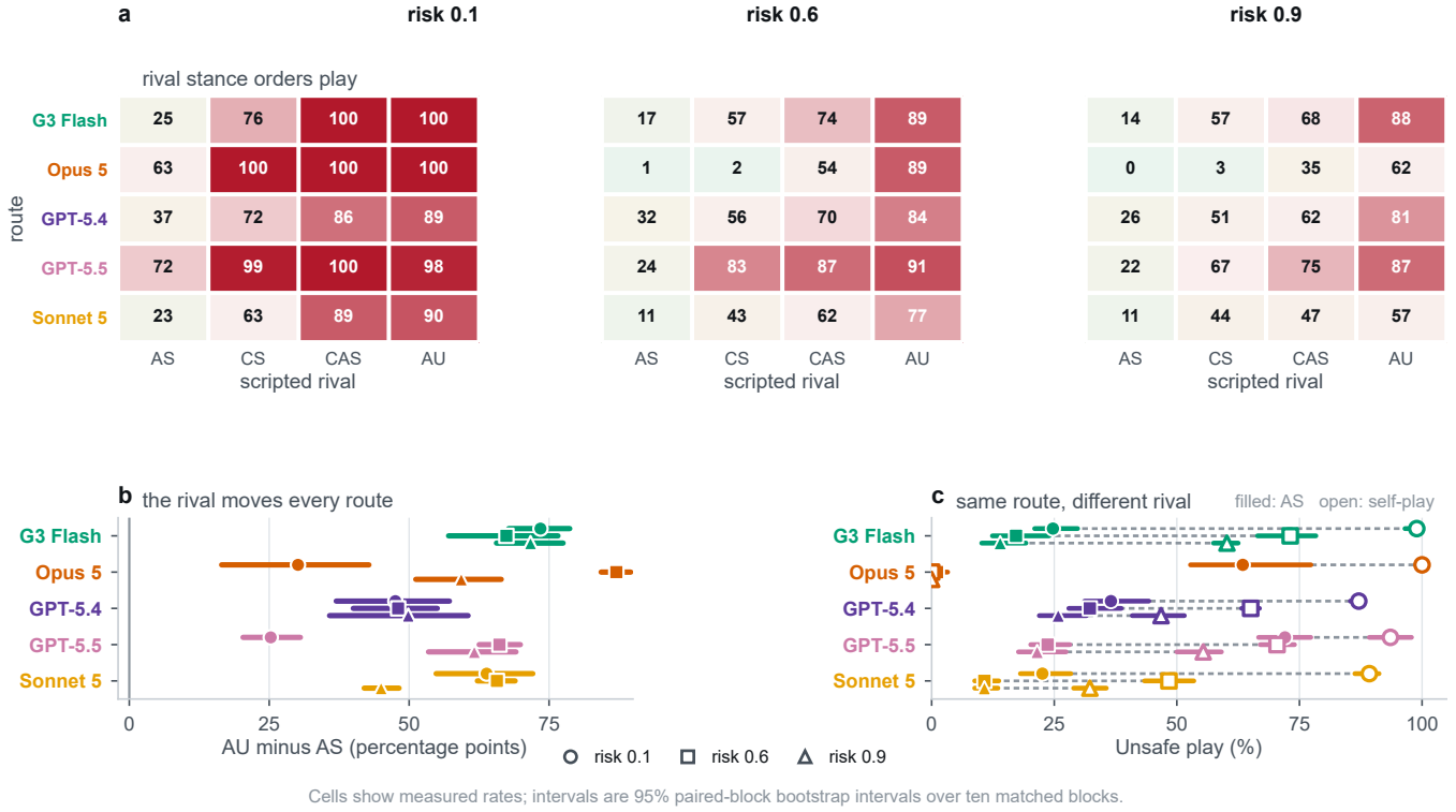
Figure 3: How the rival changes a route’s play. Panel (a) is a response surface: each tile is an admitted route’s Unsafe rate under one scripted rival, with columns ordered from Always Safe to Always Unsafe and facets for the three maximum-risk conditions. Panel (b) shows the paired Always-Unsafe minus Always-Safe effect with 95% paired-block bootstrap intervals over ten matched blocks; all fifteen effects are positive, although their magnitudes differ by route and risk. Panel (c) contrasts a fixed Always-Safe rival with self-play, separating rival-conditioned behaviour from the mirror-match outcome.
