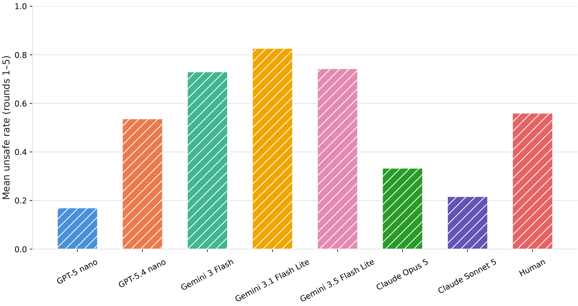
Player-level mean unsafe rate, rounds 1-5
