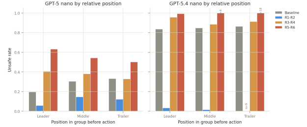
Figure 8: UNSAFE rate by relative position (Leader / Middle / Trailer) within each assigned persona band, for GPT-5-nano (left) and GPT-5.4-nano (right). Bars marked \dagger in The per-cell rates behind this figure, reported in the supplementary material, have n < 20 and should be read as noisy pilot estimates rather than stable rates.
