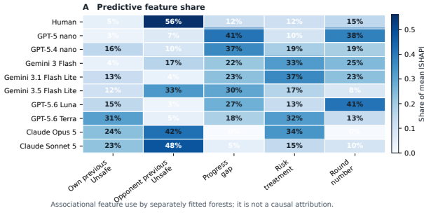
Figure 5: Population-specific predictive structure for round- t \geq 2 UNSAFE choices. Each row reports the share of mean absolute SHAP value assigned to the same five pre-decision features by a random forest fitted separately to that population. SHAP magnitudes describe how the fitted classifier uses observed features; they are neither causal effects nor evidence of the agents’ internal reasoning.
