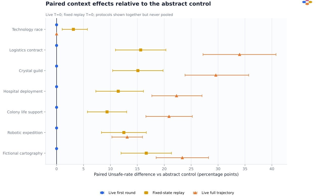
Figure 3: Exploratory temperature-zero context effects relative to the abstract control. First-round, fixed-state, and full live-trajectory contrasts answer different questions. Failed comprehension admission limits all panels to behavioral diagnostics.
