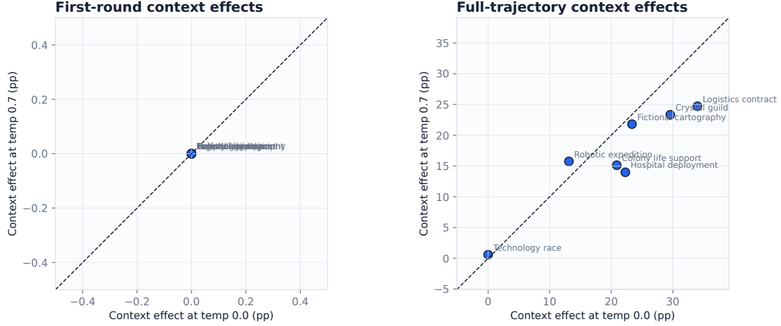
Figure 4: Full-trajectory context effects at two decoding temperatures. The diagonal indicates equality, not a causal null. Mechanism-specific hashes, first-round prompts, horizons, and model digest matched, while the whole staged-source archive hash differed; the comparison is therefore a bounded robustness diagnostic.
