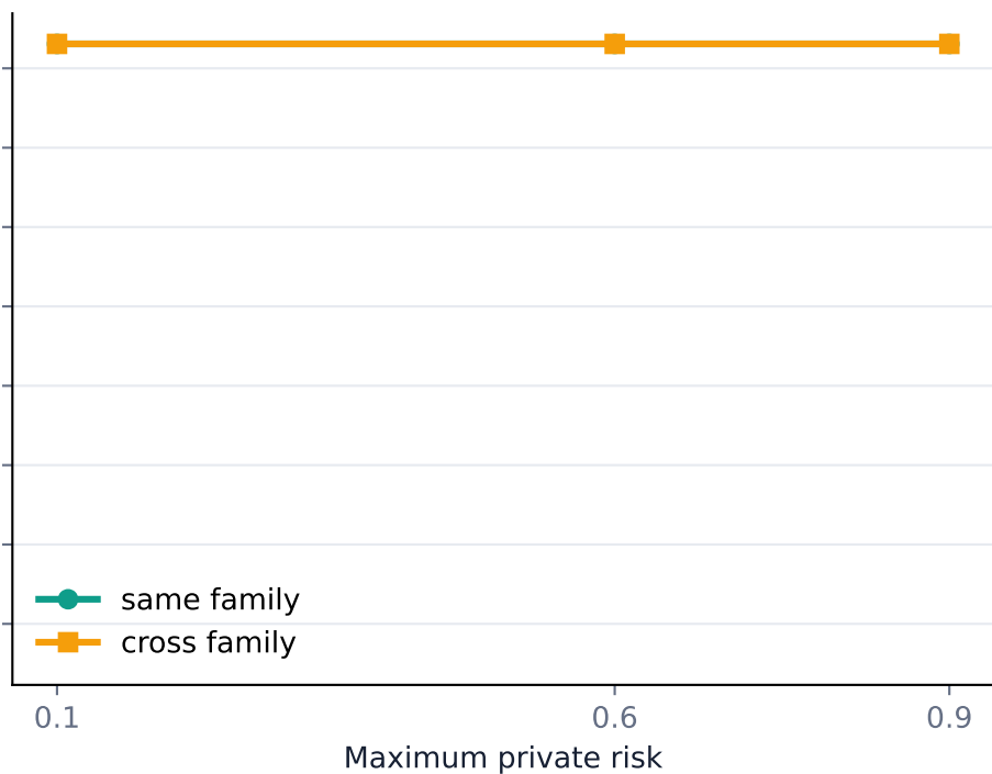
Mistral 7B
