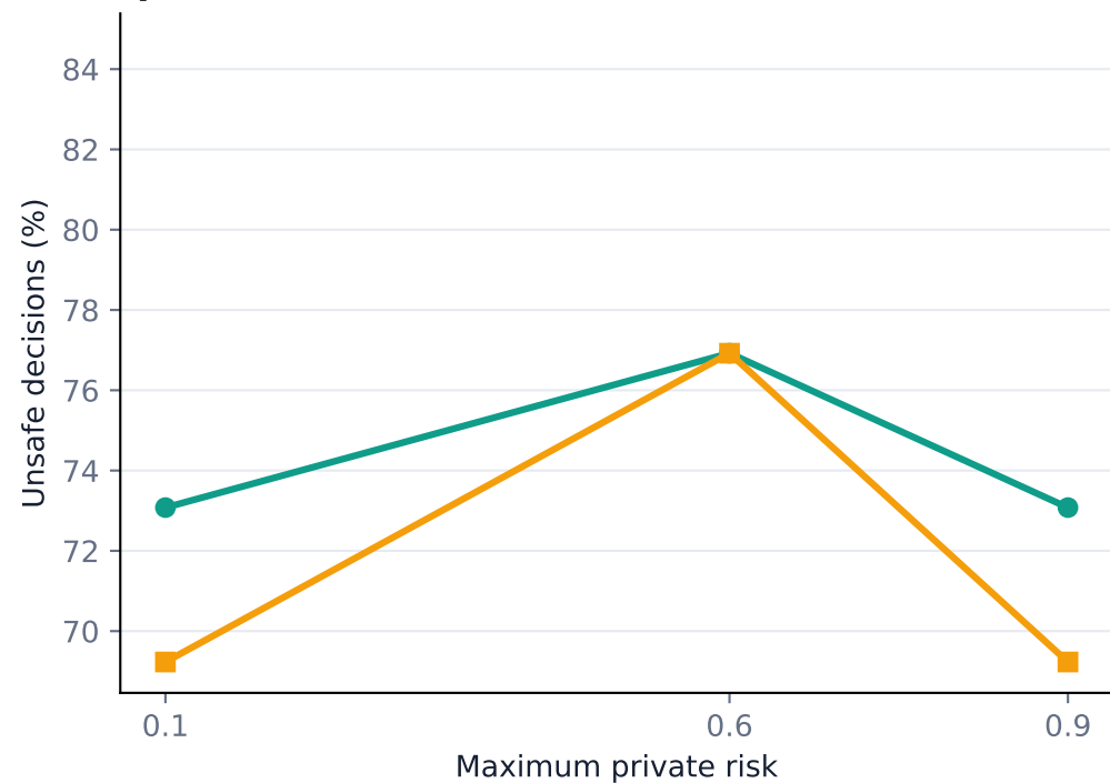
Qwen 2.5 7B
