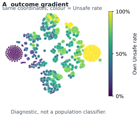
Figure 6: Outcome structure, not population identity, explains apparent regions in the pooled t-SNE. Colour and point area encode each of 760 trajectories' own Unsafe rate on fixed coordinates. This diagnostic is not a classifier, causal test or global distance measure; Figure 5 quantifies diversity.
