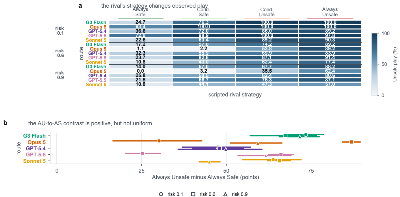
Figure 3: How the rival changes a route's play. Panel (a) is a response matrix: each row is one of five admitted routes, each risk band contains one route ordering, and the four columns are scripted rival strategies. Darker cells indicate more Unsafe play and the printed values preserve the measured rate. The strategy headers use the EGT palette, while tile shade encodes the measured Unsafe rate. Panel (b) shows the paired Always-Unsafe minus Always-Safe effect with 95% race-clustered intervals; all fifteen effects are positive, although their magnitudes differ by route and risk.
