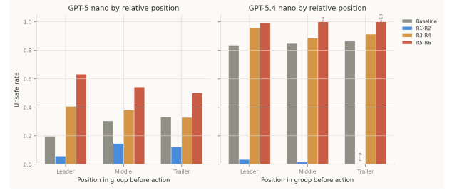
Figure 7: UNSAFE rate by relative position (Leader / Middle / Trailer) within each assigned persona band, for GPT-5-nano (left) and GPT-5.4-nano (right). Bars marked \dagger in The per-cell rates behind this figure, reported in the supplementary material, have n < 20 and should be read as noisy pilot estimates rather than stable rates.
