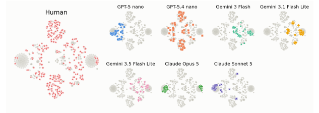
Figure 5: t-SNE visualisation of the pooled 15-dimensional raw action-and-position space. Each panel highlights one population while rendering the other populations in grey; the human sample is shown in the larger left panel, with the seven LLM checkpoints arranged smaller to its right.
