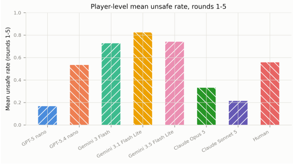
Figure 3: Player-level mean UNSAFE rate over rounds 1 to 5 per population, the numbers reported in the paragraph above.
