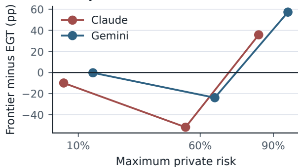
B Departure from EGT
