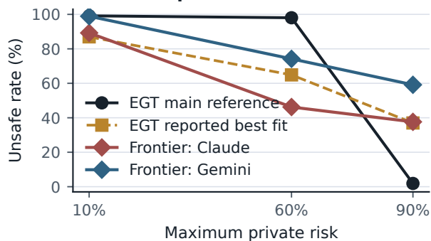
A Risk response
