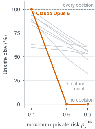
c one route is a step, not a slope
