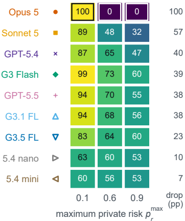
a all nine fall, by 7 to 100 points
