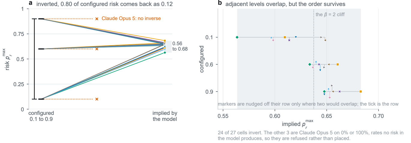
Figure 3: Inverting the reconstructed evolutionary model through the observed UNSAFE rates of the nine audited routes, at the weak-selection point \beta = 0.01 . (a) The inversion as a slope chart: configured risk on the left at full scale, the risk the model would need in order to emit the route’s observed rate on the right at the same full scale. The fan closes: 0.80 of configured risk comes back as 0.12. Claude Opus 5 has no inverse at any level, because its observed rates of 0% and 100% are rates no risk in the model produces; those three cells are refused rather than placed, and marked as refusals. (b) That band magnified, one row per configured level, with the \beta = 2 cliff marked. Adjacent rows overlap, on 0.0147 and 0.0129 of the axis, while the whole configured span of 0.80 collapses to 0.12; what the inversion loses is resolution rather than ranking, since all eight invertible routes keep the configured order and seven of the eight 0.1 cells lie strictly left of every 0.9 cell. Where two markers would fall on each other the second is nudged off its row with a leader back to it; the tick is the row. Neither panel is an estimate of a route’s perceived risk, and a compressed inverse is not an unresponsive route.
