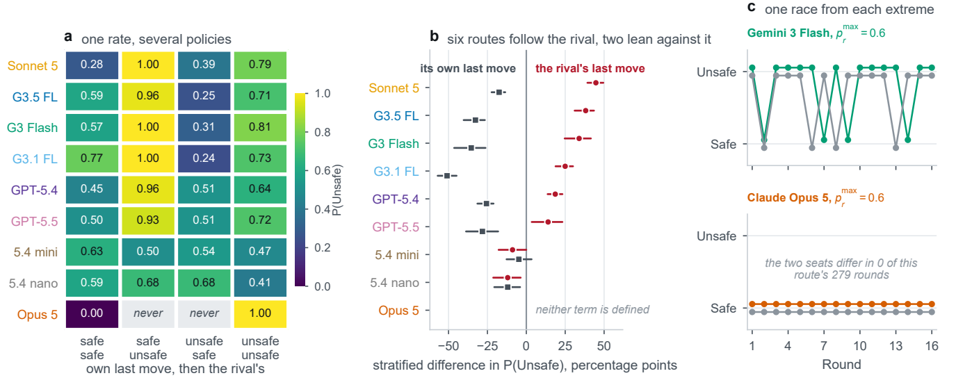
Figure 2: The memory-one policy behind each route’s UNSAFE rate, over the nine-route neutral baseline. (a) One row per route and one column per preceding pair of moves, the route’s own first and its rival’s second, with the conditional probability printed in every tile; row labels carry the route colours used throughout the paper, so the panel needs no legend. Two of Claude Opus 5’s tiles are marked absent rather than left blank: its two seats never once played differently, so the mixed contexts did not arise and there is nothing there to measure. (b) The two lagged associations on one scale, Mantel-Haenszel differences in P(\text{UNSAFE}) stratified on the risk level and on the other lagged move: how far UNSAFE play differs after the rival’s UNSAFE move, and how far it differs after the route’s own, with race-clustered 95% intervals and the routes in the same order as panel a. (c) Two races at the same risk level under the same protocol, one from a route that answers its rival and one from the route that does not move at all, with the two seats drawn separately. Every quantity here is an association within a stratum and not a causal effect. Nothing is randomised: these are conditional frequencies from nine commercial endpoints in one game at one prompt version, self-play throughout, and the own term in particular also carries the accumulated private risk that an earlier UNSAFE move leaves behind, so it is a response to the state and not to the move alone.
