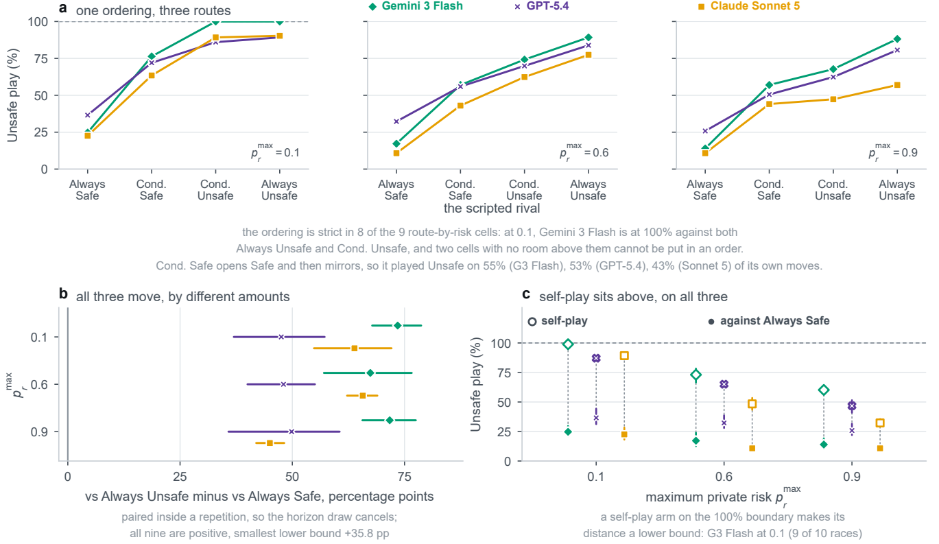
Figure 14: The scripted-opponent campaign on three gate-admitted routes. (a) The ordering, one facet per stated risk: four rivals across, the route’s own UNSAFE play up. A rising line is the ordering, and the vertical distance between the three lines is how far the routes differ in level. (b) The rival-stance contrast, the rate against Always Unsafe minus the rate against Always Safe , differenced inside a repetition so that the horizon stopping draw is removed. All nine intervals lie to the right of zero, and the three routes separate. (c) The comparison the tables cannot make: each route’s rate against a rival that stays SAFE, as a filled marker, beside the rate the same route reaches when its rival is a second copy of itself, as an open marker.
