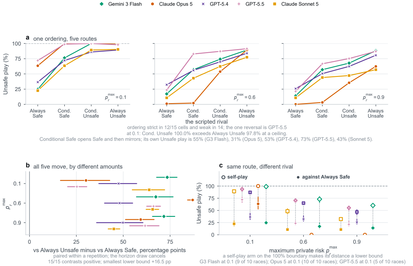
Figure 15: The scripted-opponent campaign on five gate-admitted routes. (a) The ordering, one facet per stated risk: four rivals across, the route’s own UNSAFE play up. A rising line is the ordering, and the vertical distance between the five lines is how far the routes differ in level. (b) The rival-stance contrast, the rate against Always Unsafe minus the rate against Always Safe , differenced inside a repetition so that the horizon stopping draw is removed. All fifteen intervals lie to the right of zero, with magnitudes that differ by route. (c) The comparison the tables cannot make: each route’s rate against a rival that stays SAFE, as a filled marker, beside the rate the same route reaches when its rival is a second copy of itself, as an open marker.
