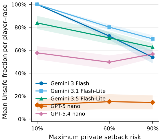
A Risk response differs sharply across models
