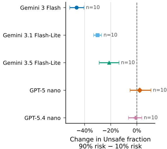
B Paired repetition-block contrast
