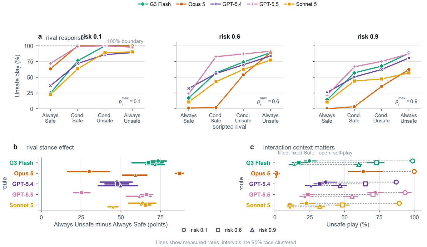
Figure 15: The scripted-opponent campaign on five gate-admitted routes. (a) The ordering, one facet per stated risk: four rivals across, the route’s own UNSAFE play up. A rising line is the ordering, and the vertical distance between the five lines is how far the routes differ in level. (b) The rival-stance contrast, the rate against Always Unsafe minus the rate against Always Safe , differenced inside a repetition so that the horizon stopping draw is removed. All fifteen intervals lie to the right of zero, with magnitudes that differ by route. (c) The comparison the tables cannot make: each route’s rate against a rival that stays SAFE , as a filled marker, beside the rate the same route reaches when its rival is a second copy of itself, as an open marker.
