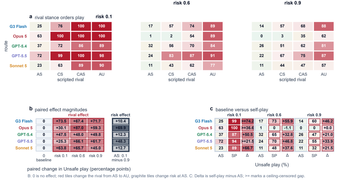
Figure 5: The scripted-opponent campaign on five gate-admitted routes. (a) Response surfaces across scripted rivals and stated-risk levels. (b) Paired effect magnitudes: the Always-Unsafe minus Always-Safe rival effect at each risk, with the fixed-safe risk effect shown on the same percentage-point scale. (c) Always-Safe rates, self-play rates and their signed differences; a \geq label marks a ceiling-censored gap. Confidence intervals for the rival contrast are reported in Table 11.
