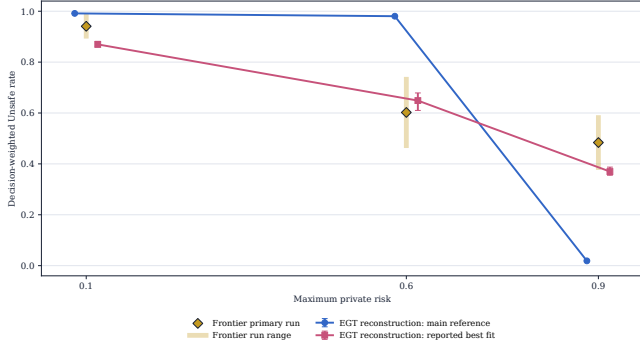
Figure 3: Frontier Unsafe decisions against the reconstructed evolutionary benchmark. The theory curves are stationary strategy mixtures; the frontier ranges and pooled points summarise two admitted routes, each with 30 completed races. Independent-chain ranges are shown for the theory reconstruction.
