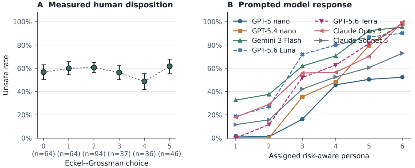
Figure 6: A measured human disposition against an assigned model label. Left: mean UNSAFE rate by elicited Eckel–Grossman gamble choice, with 95% confidence intervals and participants per bin; the dotted line is the trend across the six group means. Right: mean UNSAFE rate by assigned risk-persona level, for every model with a six-level sweep; GPT-5.6 Luna and Terra (dashed) are the two routes outside the main baseline roster. The shared six-step axis is visual alignment only; the left is a disposition measured once before play, the right an instruction re-assigned every race.
