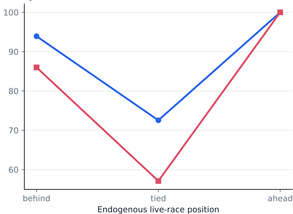
Qwen 2.5 7B
