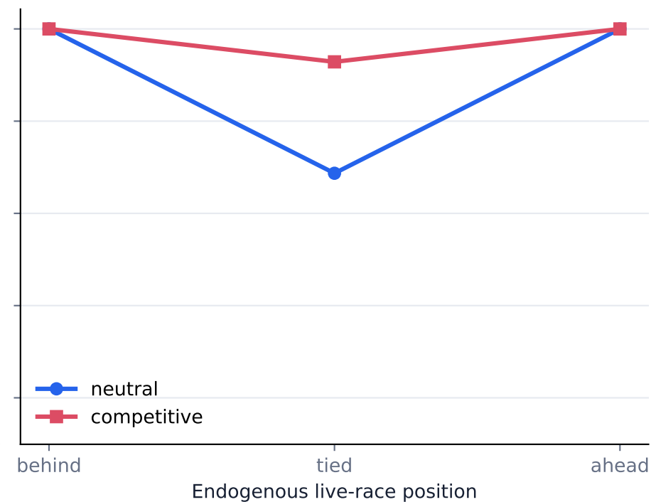
Mistral 7B
