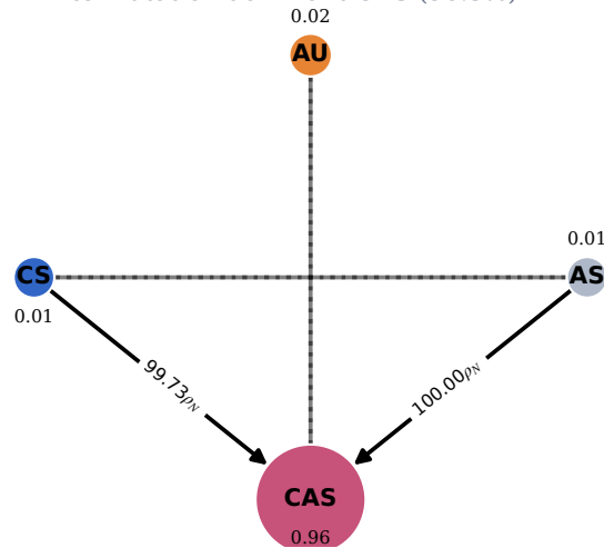
b r_{\max} = 0.6 finite-mutation dominant CAS (96.3%)
