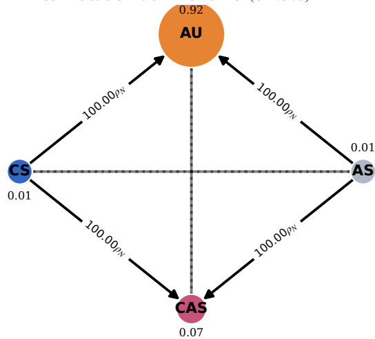
a r_{\max} = 0.1 finite-mutation dominant AU (91.9%)
