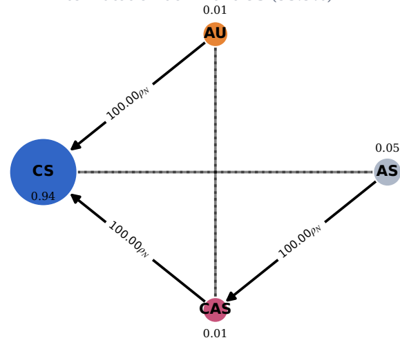
c r_{\max} = 0.9 finite-mutation dominant CS (93.9%)
