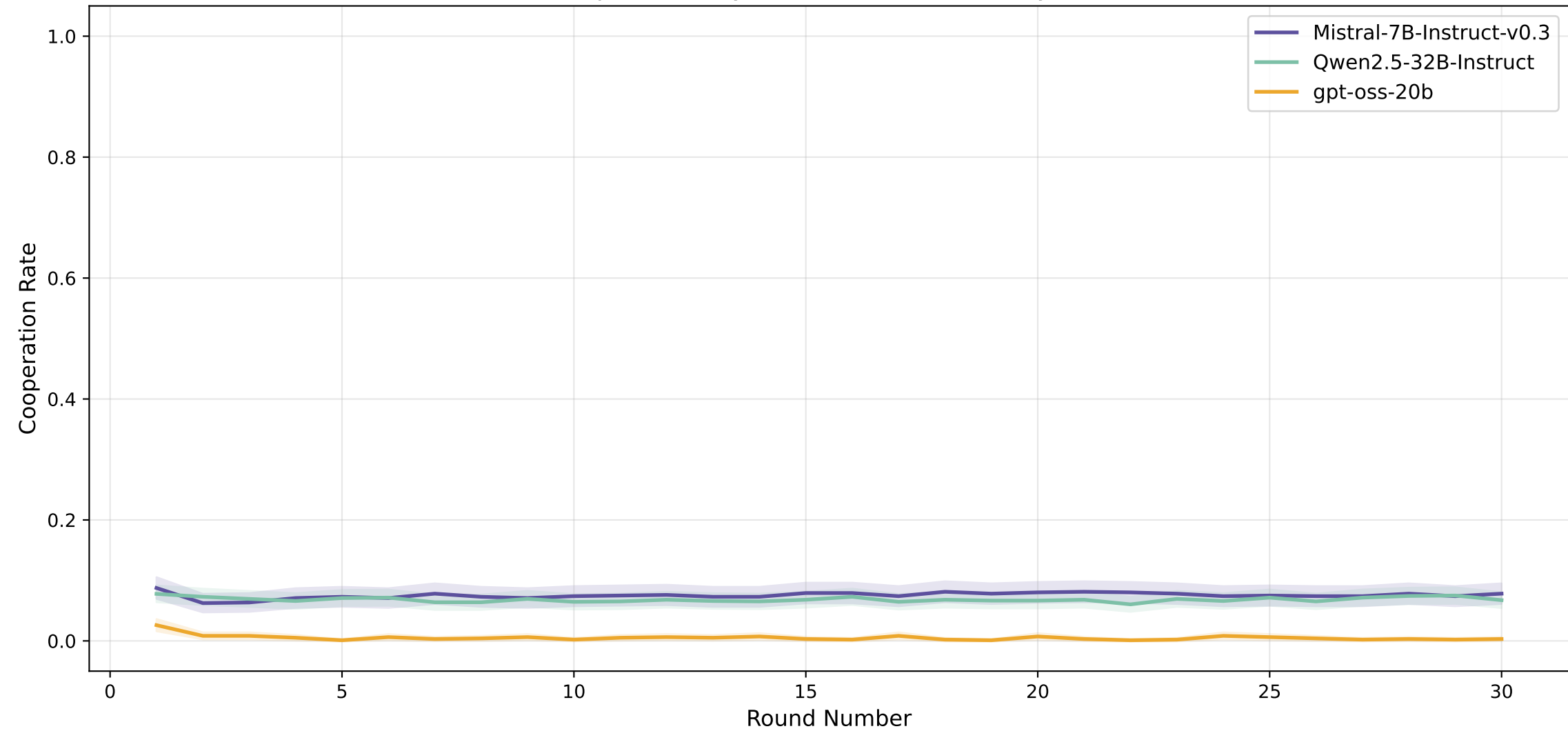
Cooperation Dynamics Over Rounds by LLM
