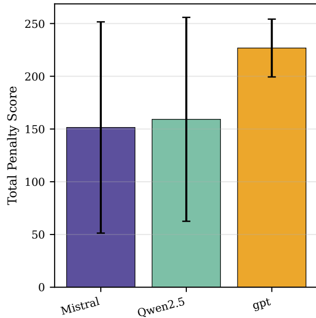
Penalty by LLM
