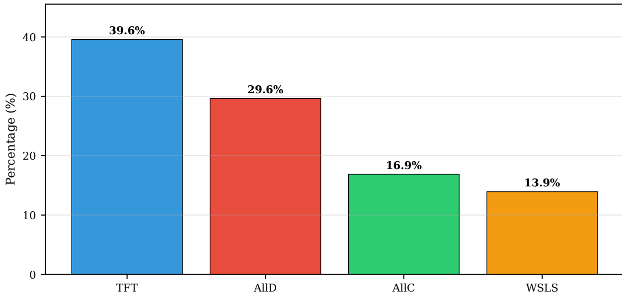
Overall Strategy Distribution (2-Player PD)
