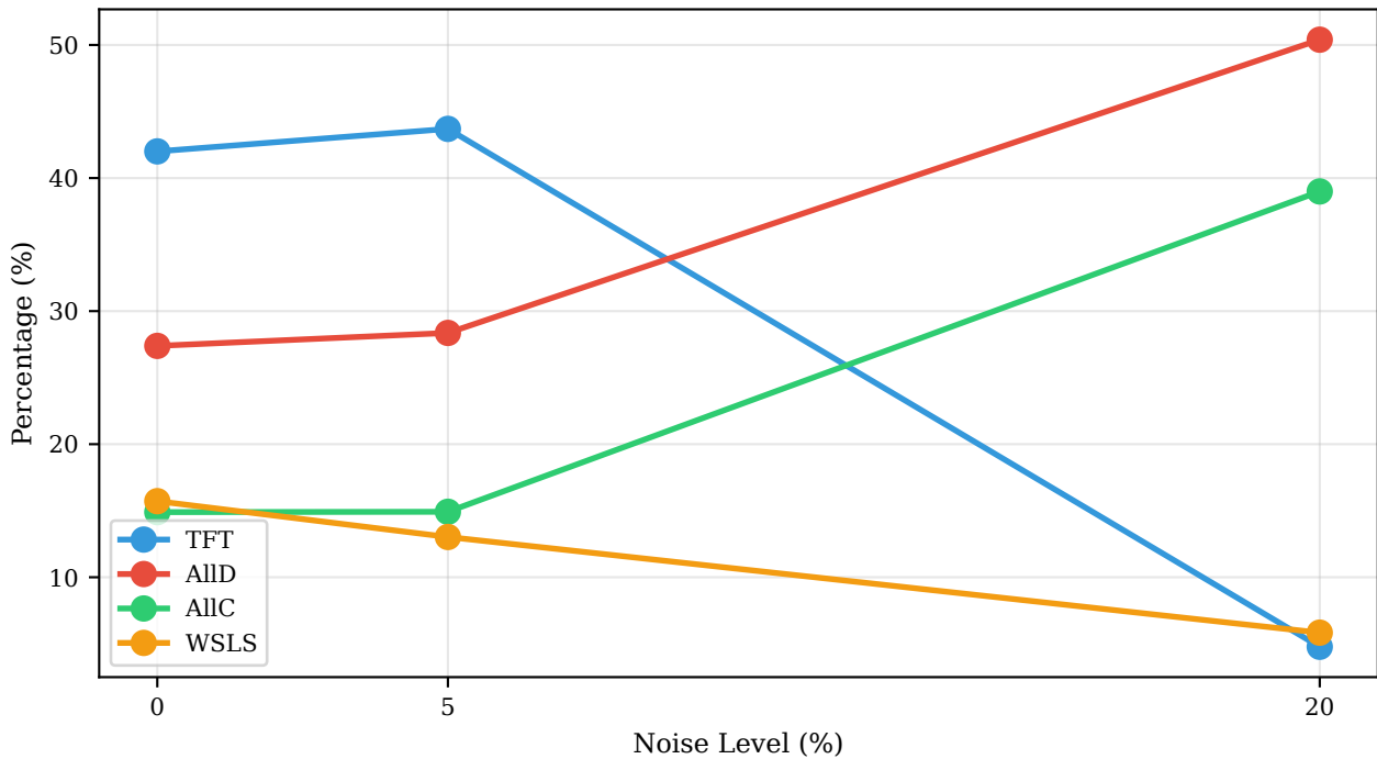
Strategy Distribution Trends by Noise Level
