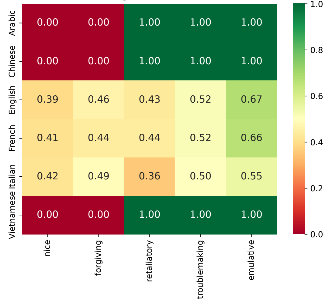
Qwen-32B
