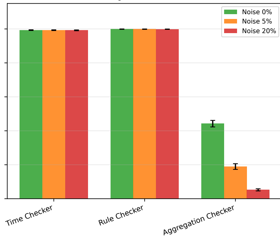
Qwen-32B
