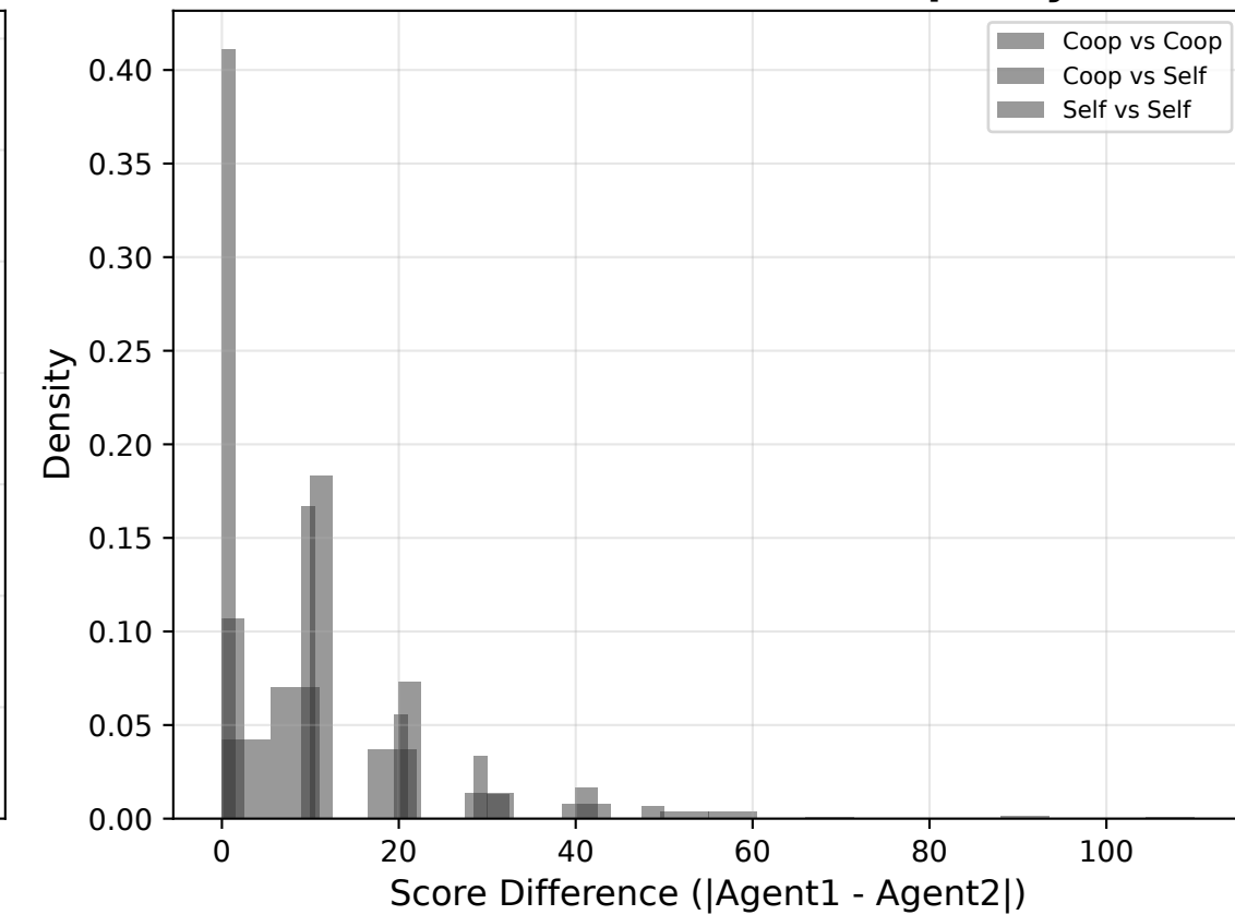
GPT-oss-20B — Score Inequality
