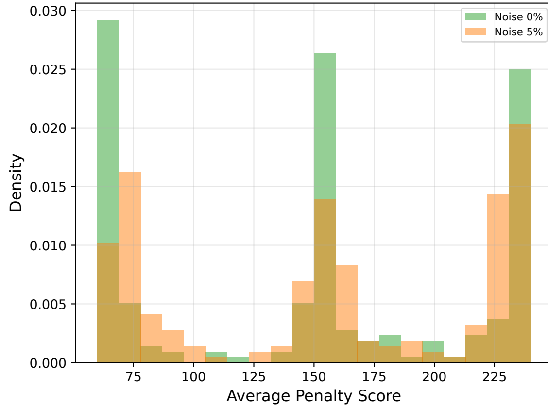
Mistral-7B — Score Inequality
