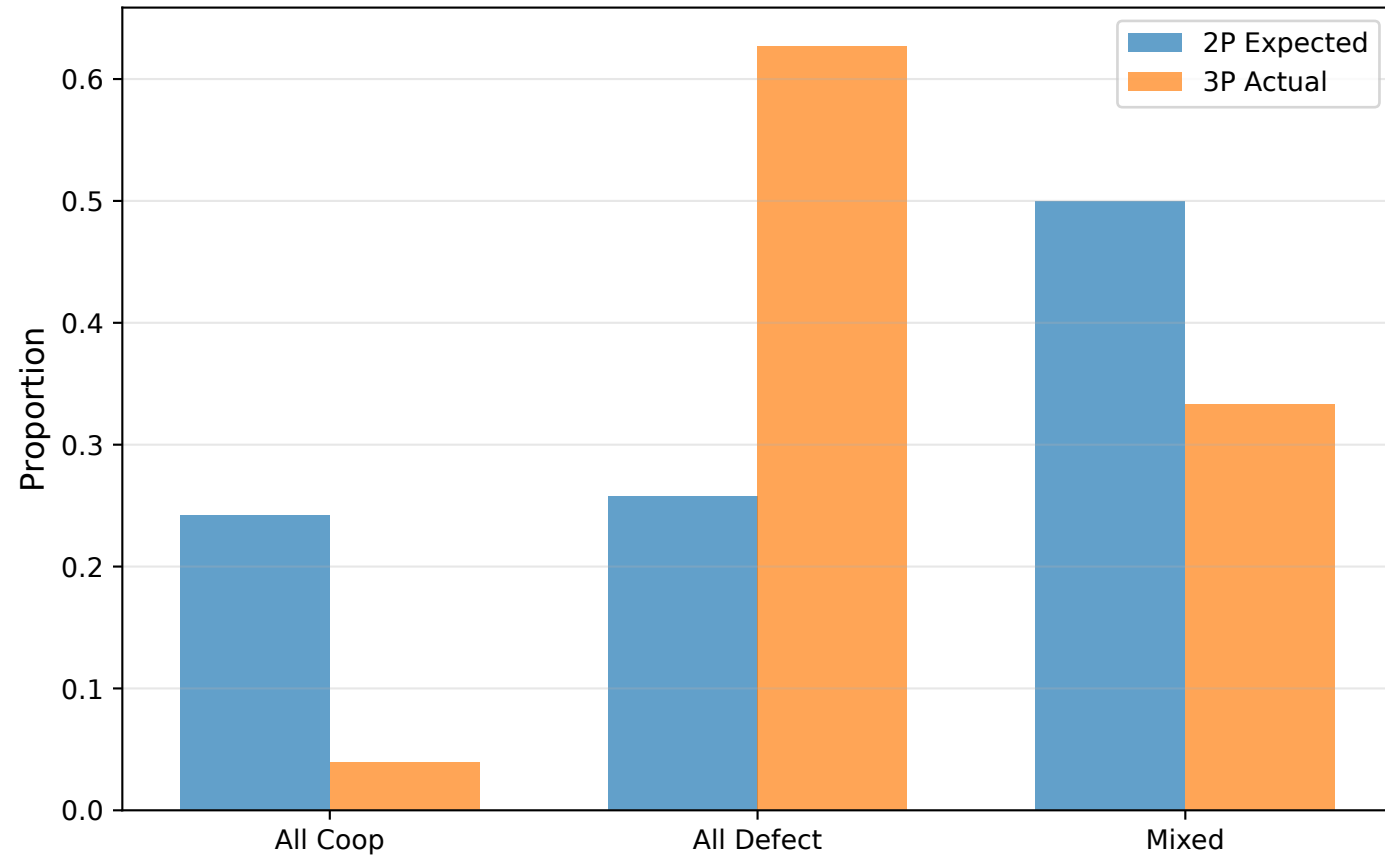
2P vs 3P State Distribution (Mistral-7B)
