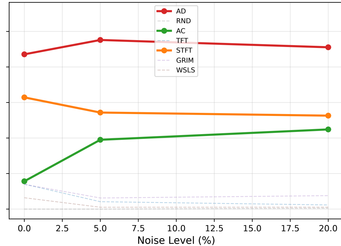
Qwen-32B
