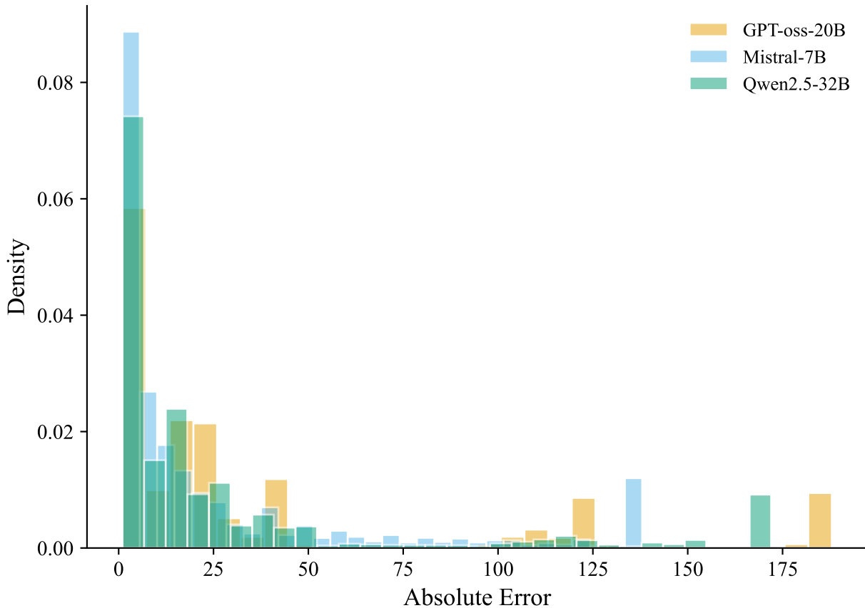
(a) Error Magnitude Distribution
