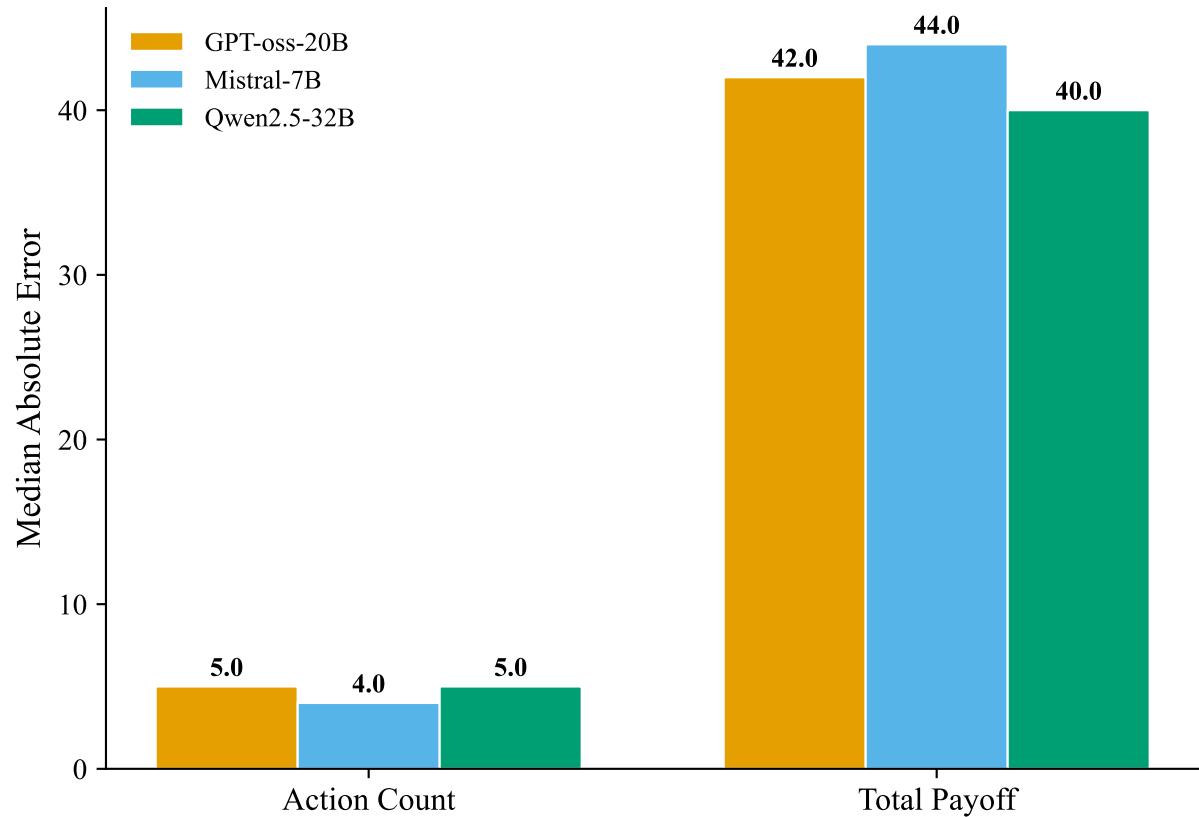
(b) Median Error by Task Type
