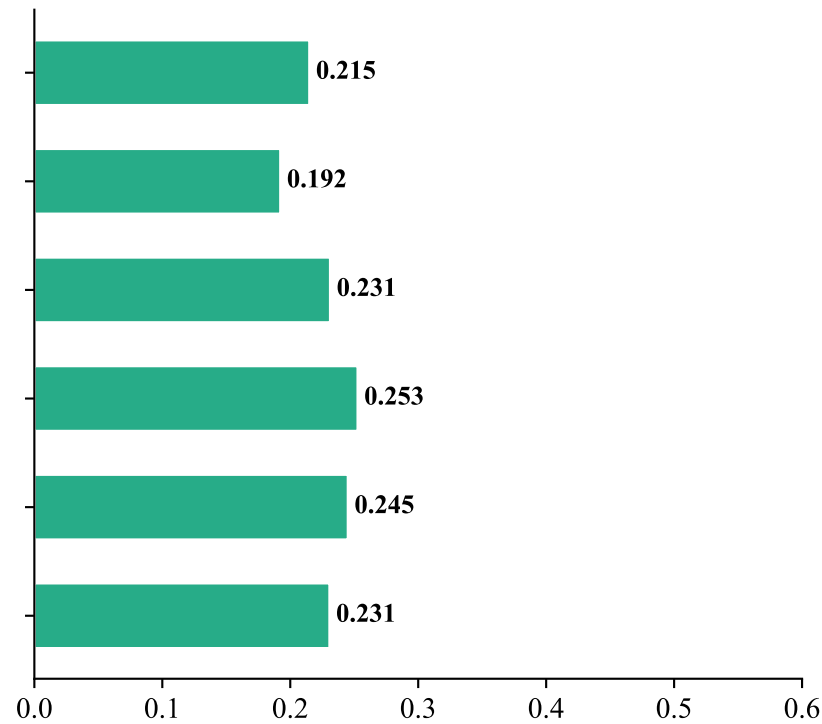
Qwen2.5-32B
