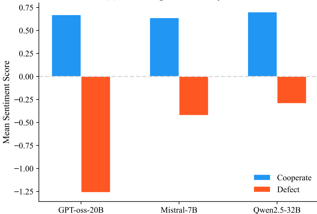
(a) Reasoning Sentiment by Action
