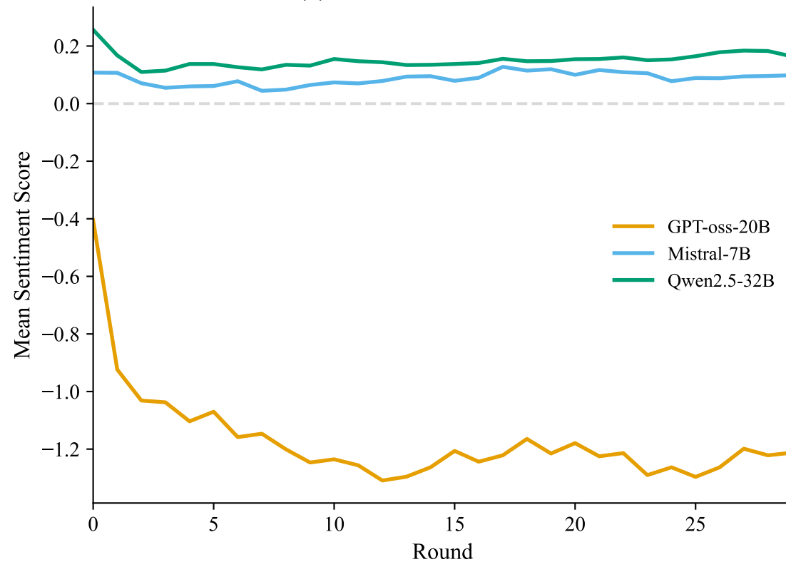
(b) Sentiment Over Rounds
